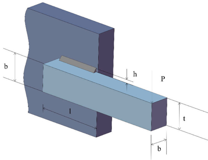
Fig. 13. WBD problem.
